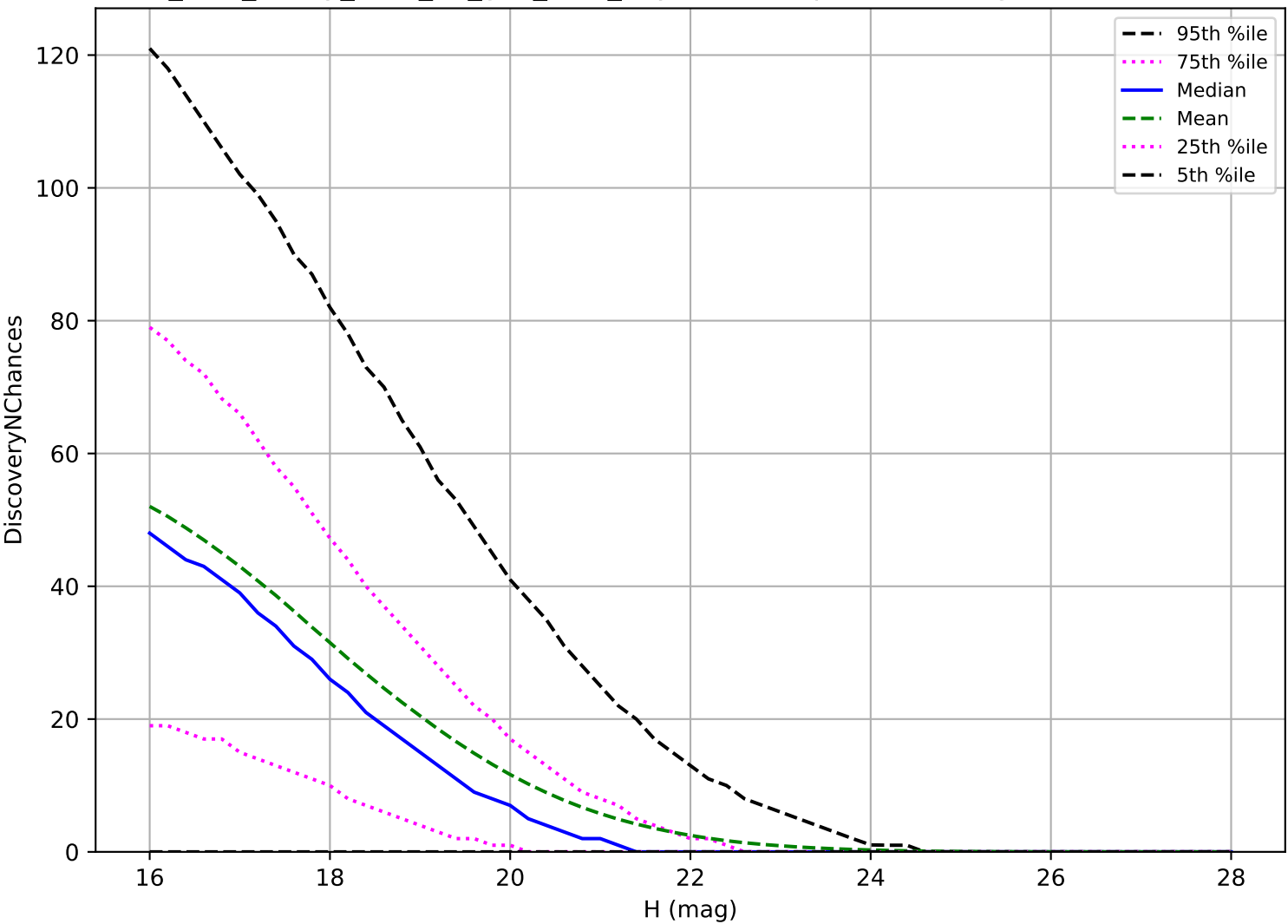
too_elab_heavy_r128_d2_griz_v3.4_10yrs: NEO 3 pairs in 15 nights detection loss
