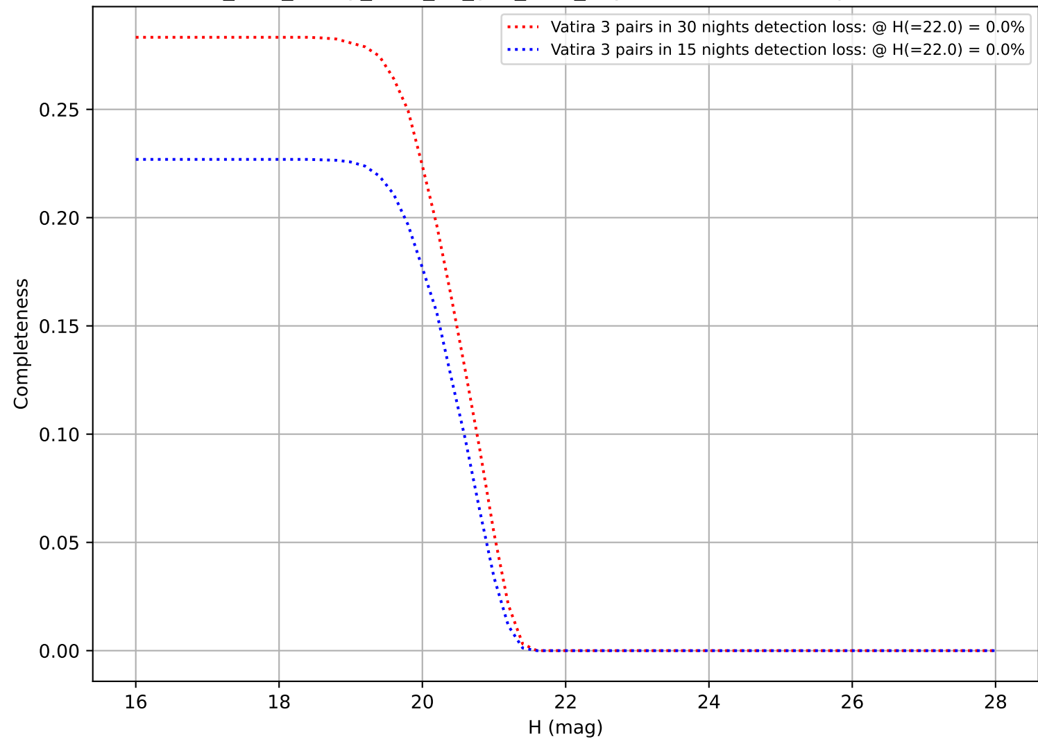
too_elab_heavy_r128_d2_griz_v3.4_10yrs: DifferentialCompleteness
