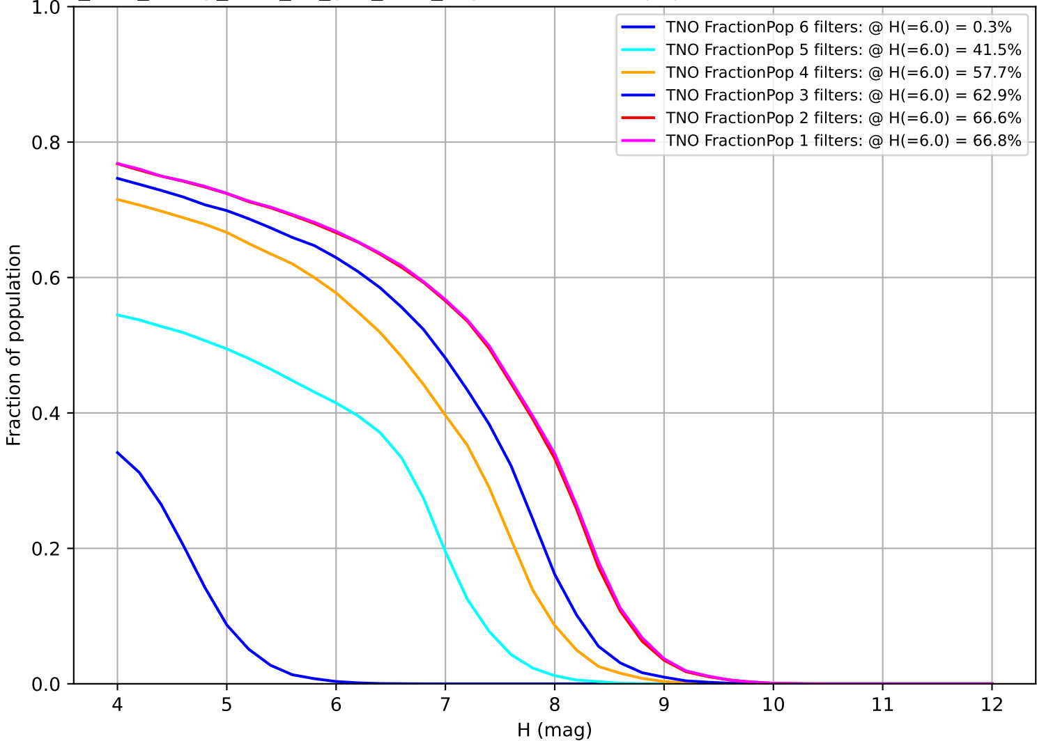
too_elab_heavy_r128_d2_griz_v3.4_10yrs: Fraction of population with colors in X filters TNO
