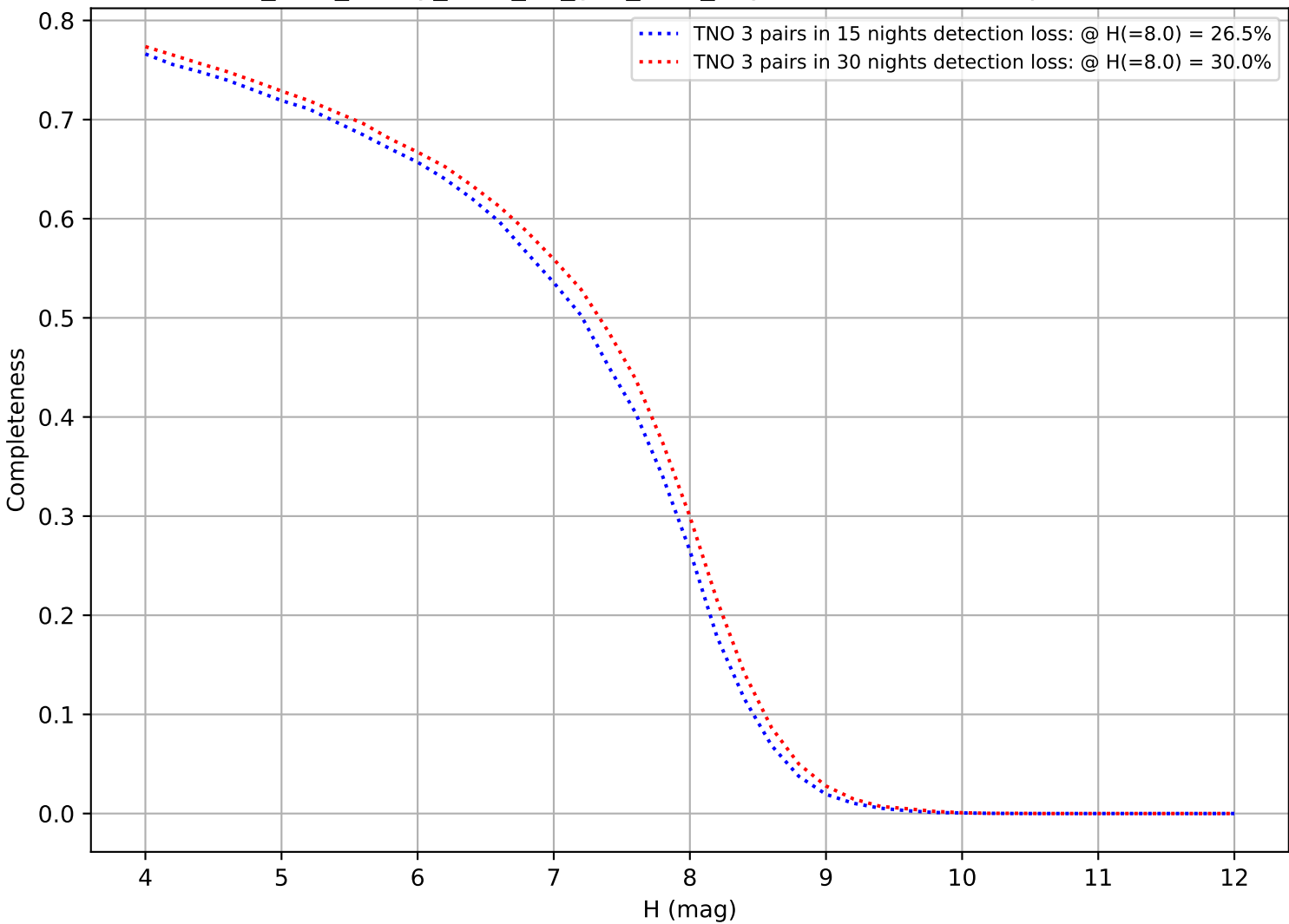
too_elab_heavy_r128_d2_griz_v3.4_10yrs: DifferentialCompleteness
