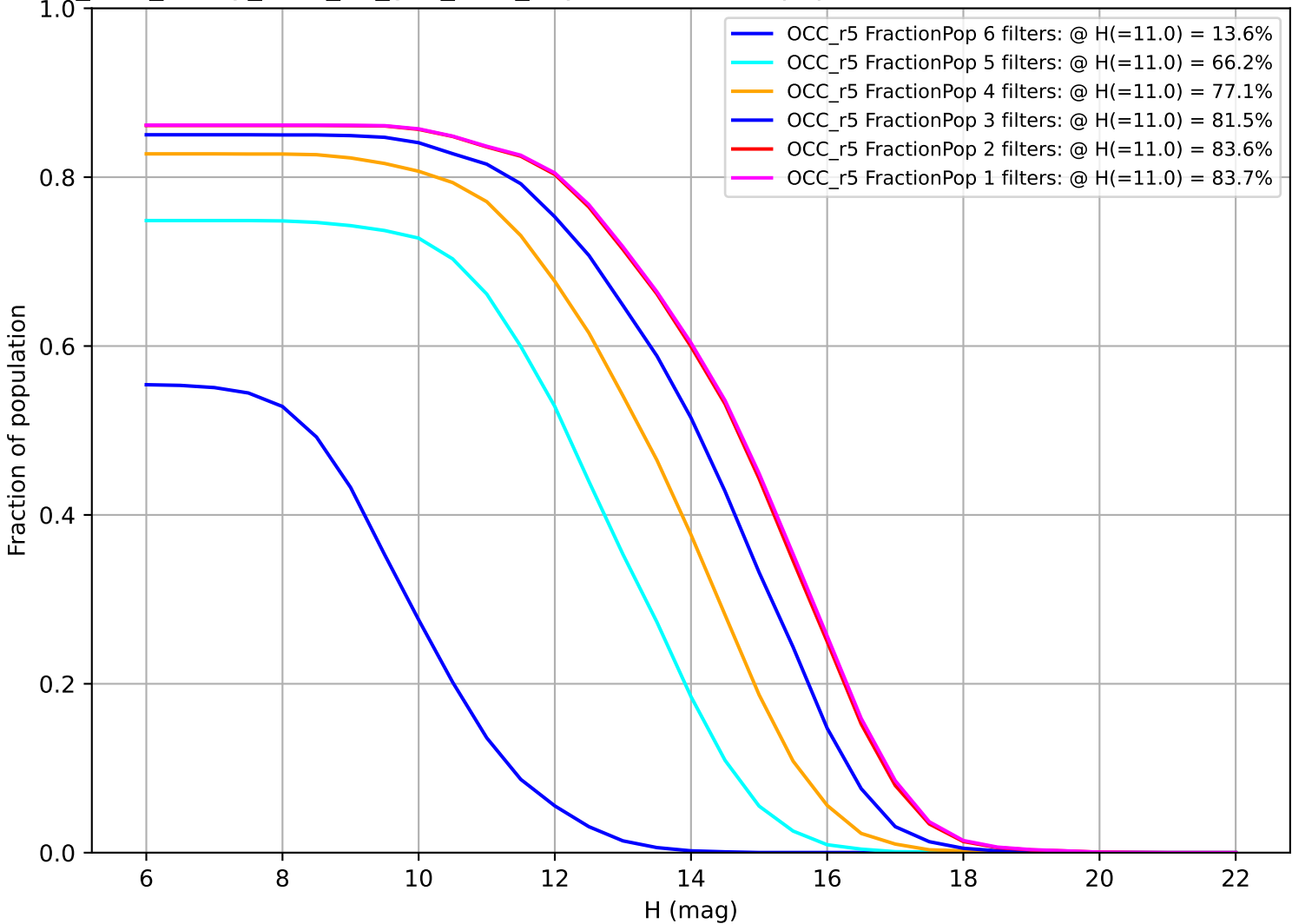
too_elab_heavy_r128_d2_griz_v3.4_10yrs: Fraction of population with colors in X filters OCC_r5
