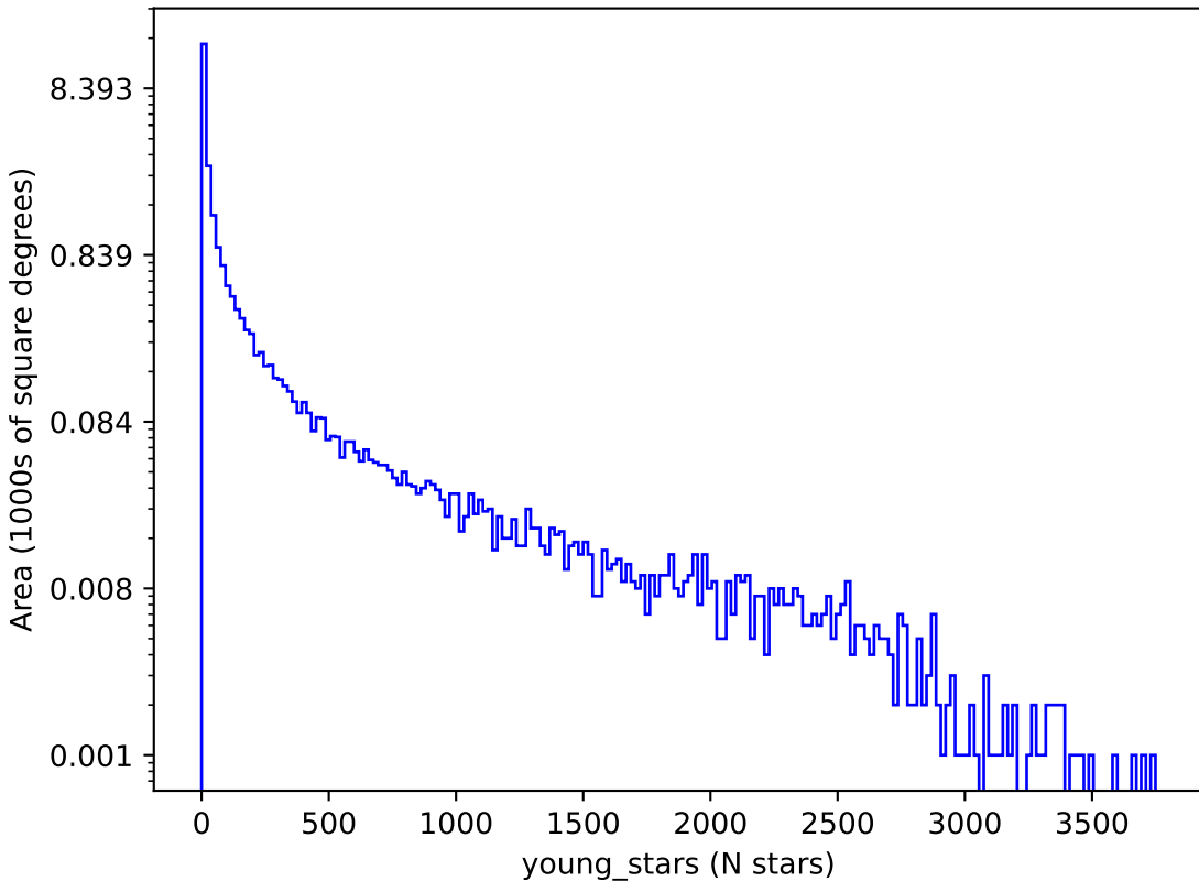
too_elab_heavy_r128_d2_griz_v3.4_10yrs : young_stars
