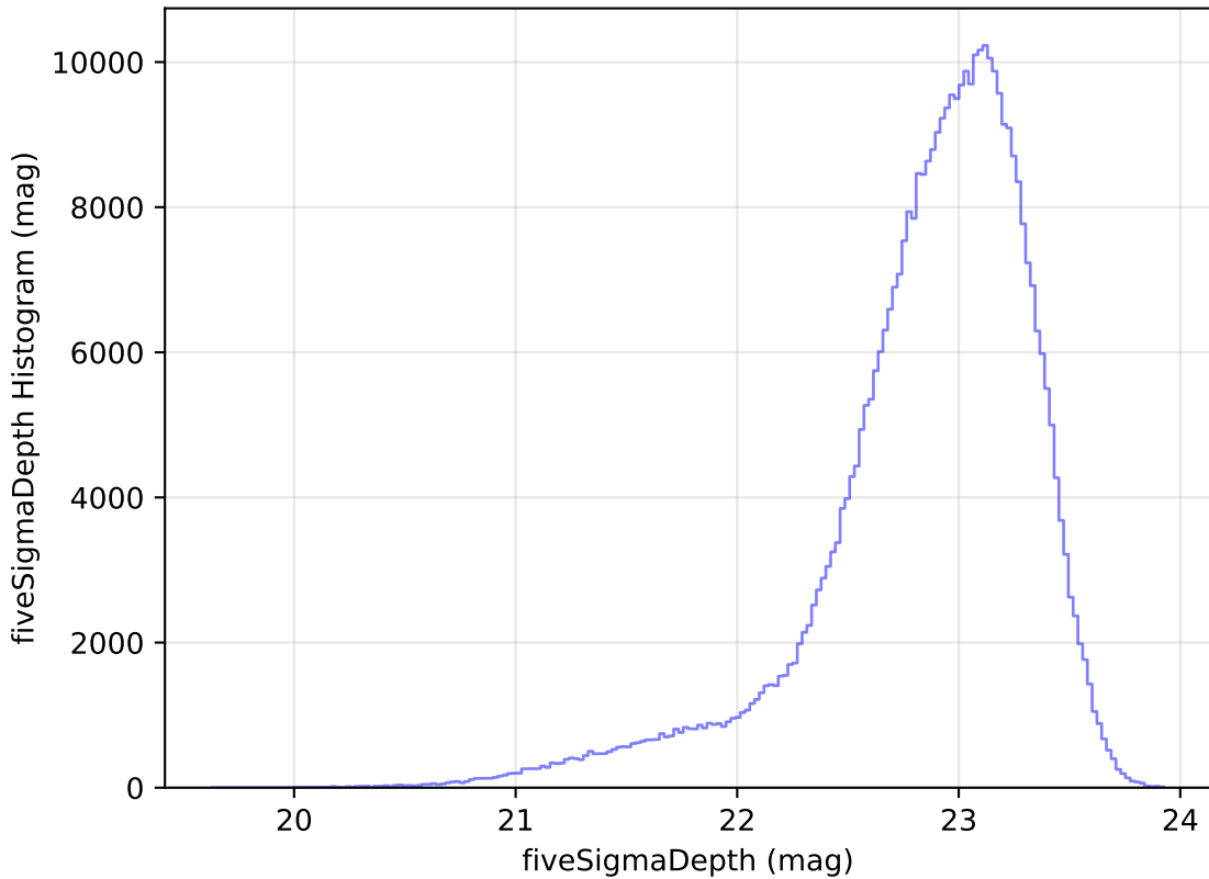
too_elab_heavy_r128_d2_griz_v3.4_10yrs z: fiveSigmaDepth Histogram
