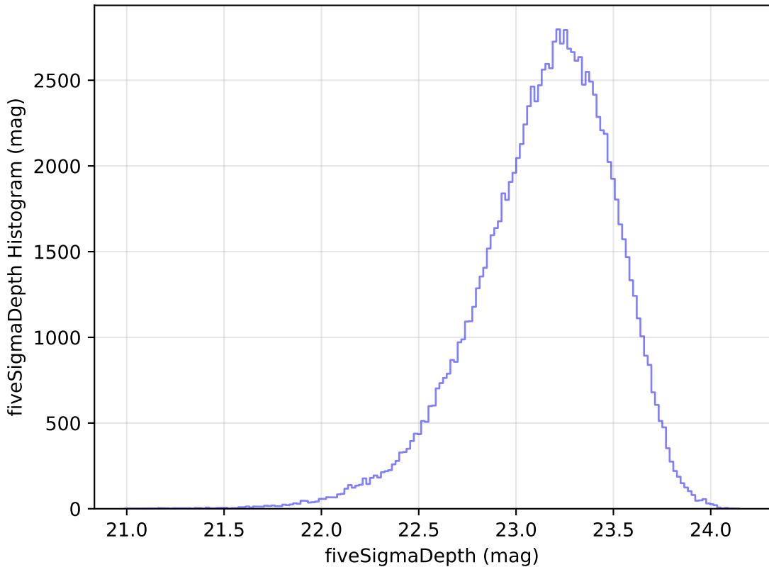
too_elab_heavy_r128_d2_griz_v3.4_10yrs u: fiveSigmaDepth Histogram
