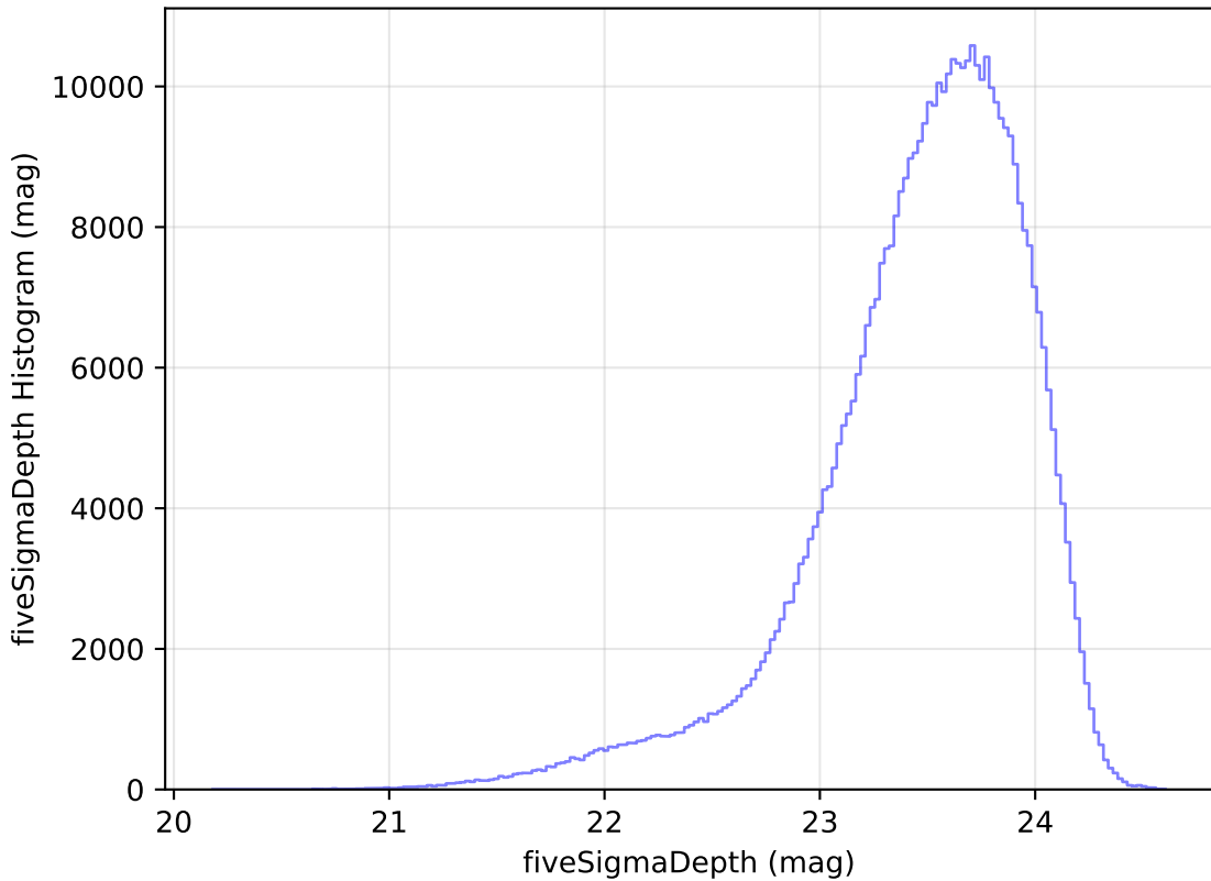
too_elab_heavy_r128_d2_griz_v3.4_10yrs i: fiveSigmaDepth Histogram
