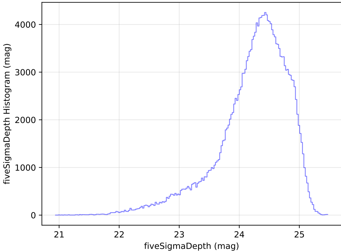
too_elab_heavy_r128_d2_griz_v3.4_10yrs g: fiveSigmaDepth Histogram
