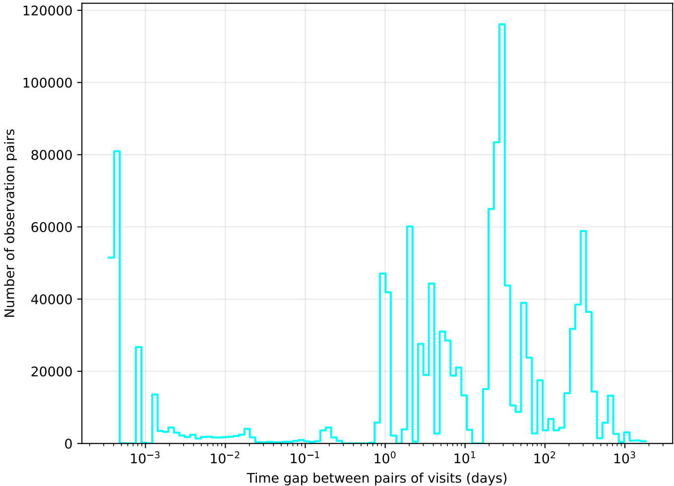
too_elab_heavy_r128_d2_griz_v3.4_10yrs u band: Tgaps observationStartMJD
