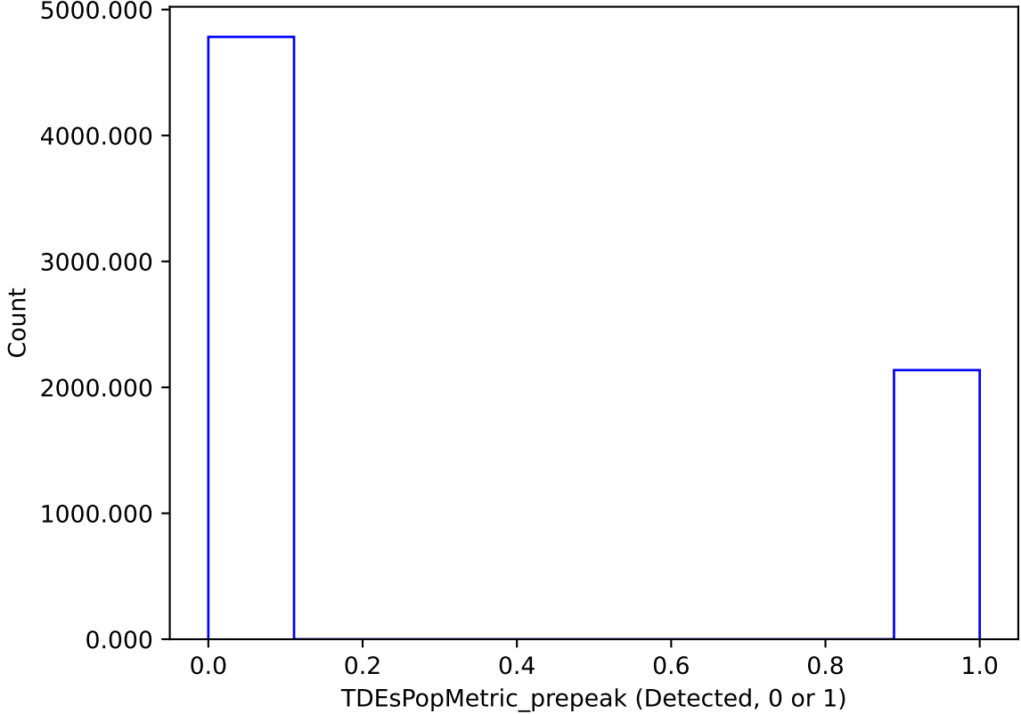
too_elab_heavy_r128_d2_griz_v3.4_10yrs : TDEsPopMetric_prepeak
