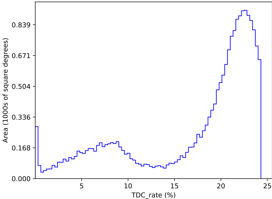
too_elab_heavy_r128_d2_griz_v3.4_10yrs : TDC_rate
