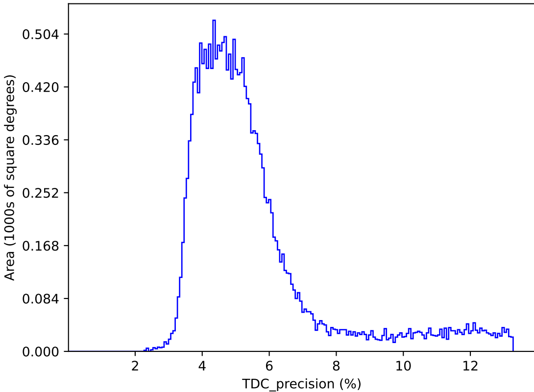
too_elab_heavy_r128_d2_griz_v3.4_10yrs : TDC_precision
