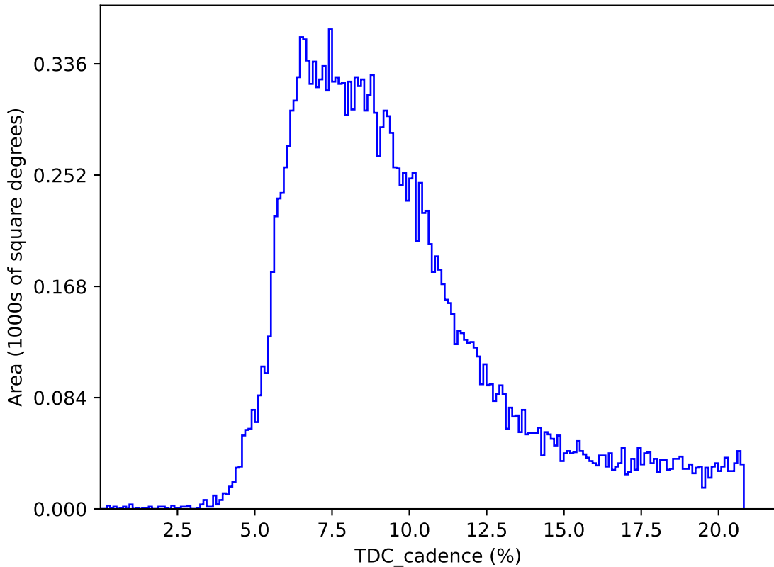
too_elab_heavy_r128_d2_griz_v3.4_10yrs : TDC_cadence
