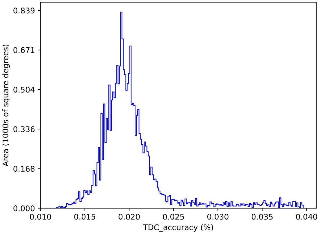
too_elab_heavy_r128_d2_griz_v3.4_10yrs : TDC_accuracy
