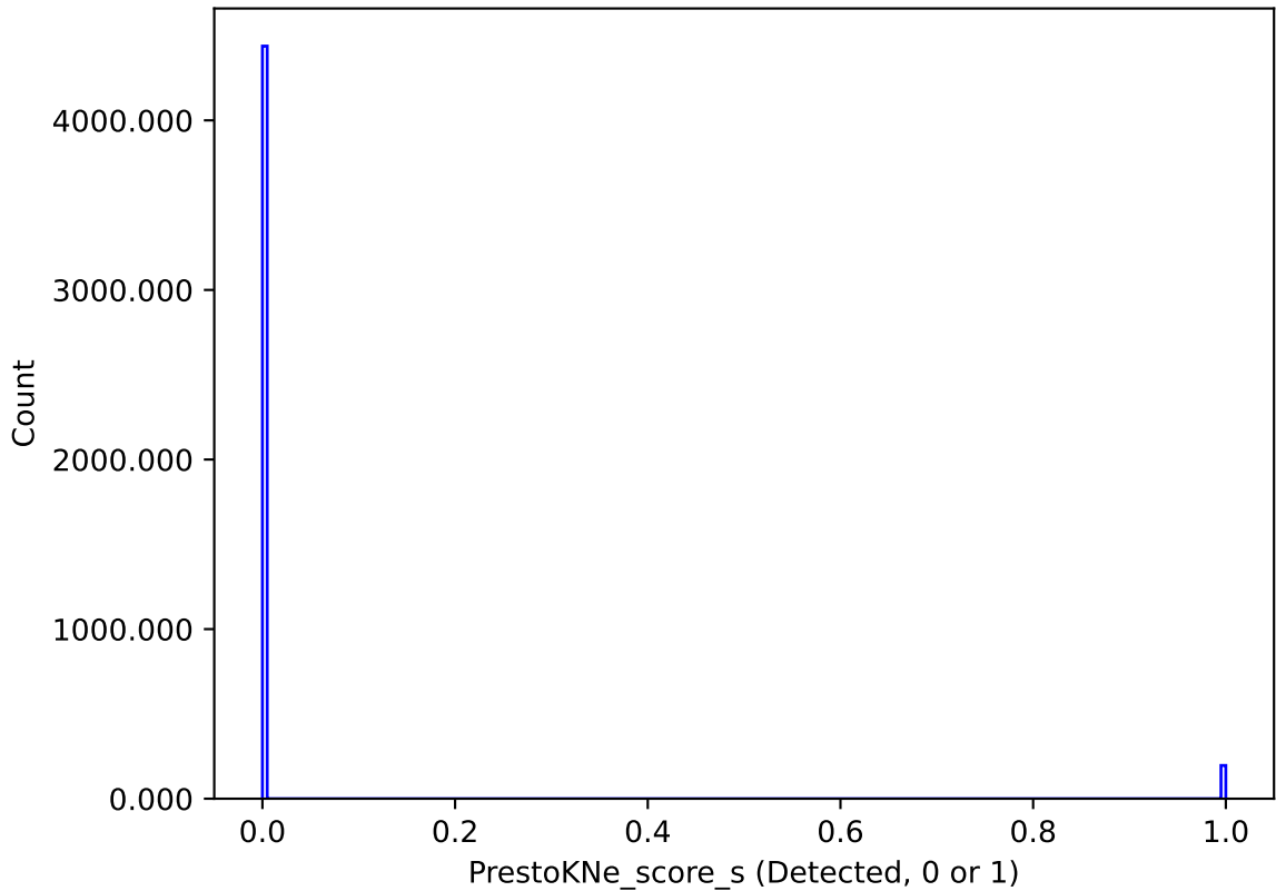
too_elab_heavy_r128_d2_griz_v3.4_10yrs : PrestoKNe_score_s
