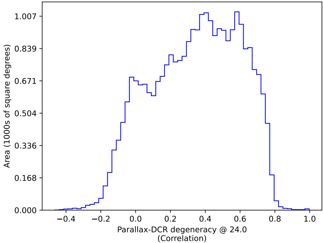
too_elab_heavy_r128_d2_griz_v3.4_10yrs : Parallax-DCR degeneracy @ 24.0
