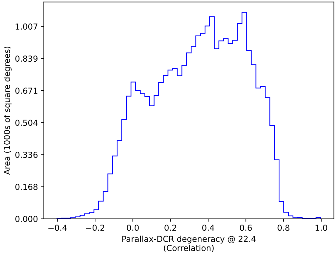
too_elab_heavy_r128_d2_griz_v3.4_10yrs : Parallax-DCR degeneracy @ 22.4
