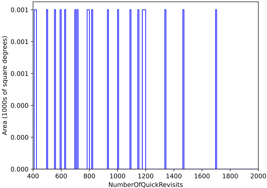
too_elab_heavy_r128_d2_griz_v3.4_10yrs : NumberOfQuickRevisits
