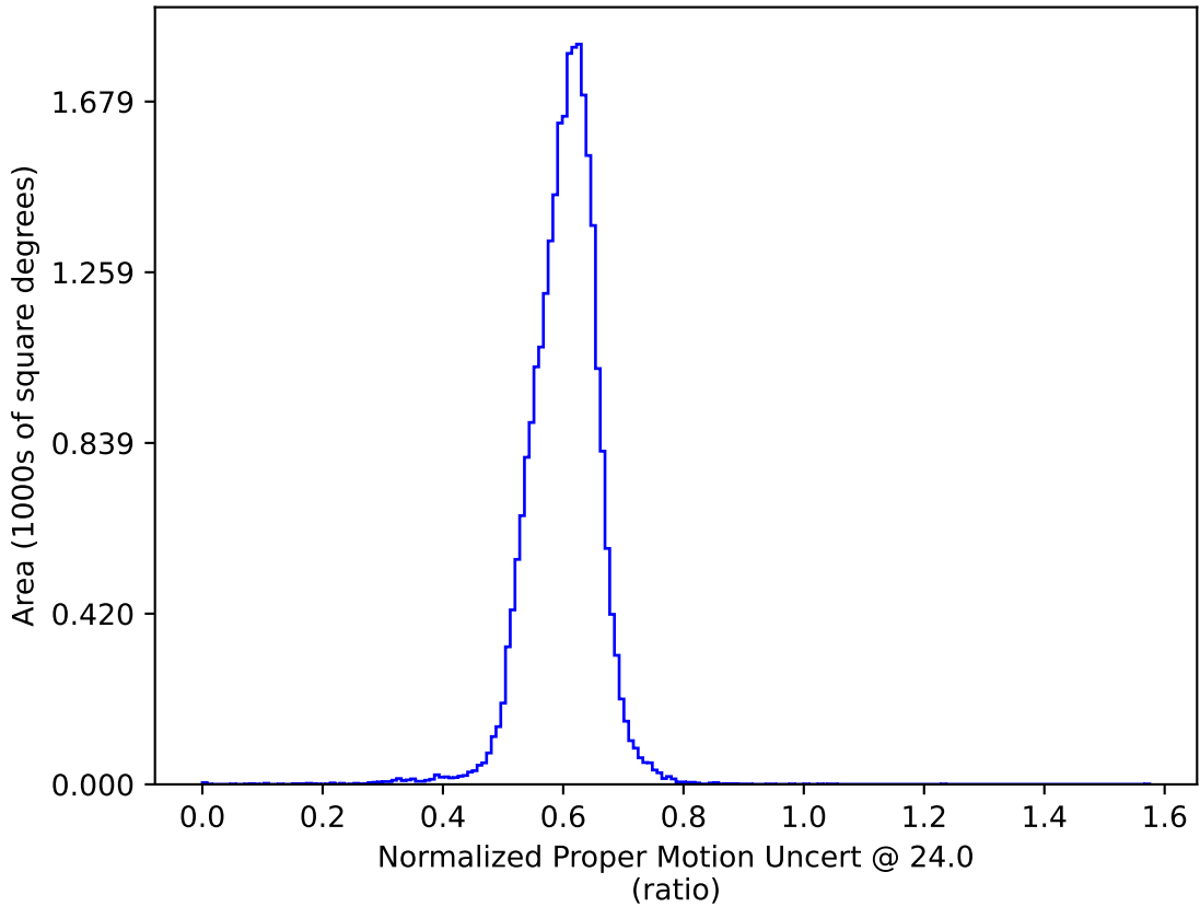
too_elab_heavy_r128_d2_griz_v3.4_10yrs : Normalized Proper Motion Uncert @ 24.0
