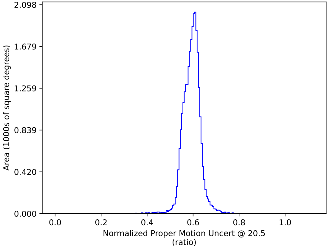
too_elab_heavy_r128_d2_griz_v3.4_10yrs : Normalized Proper Motion Uncert @ 20.5
