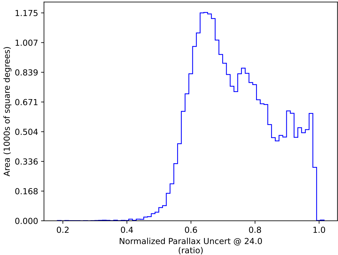
too_elab_heavy_r128_d2_griz_v3.4_10yrs : Normalized Parallax Uncert @ 24.0
