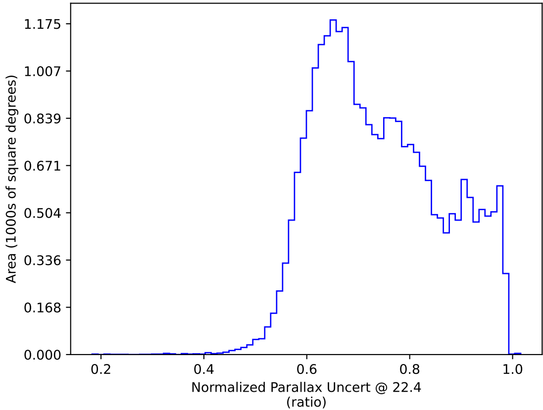
too_elab_heavy_r128_d2_griz_v3.4_10yrs : Normalized Parallax Uncert @ 22.4
