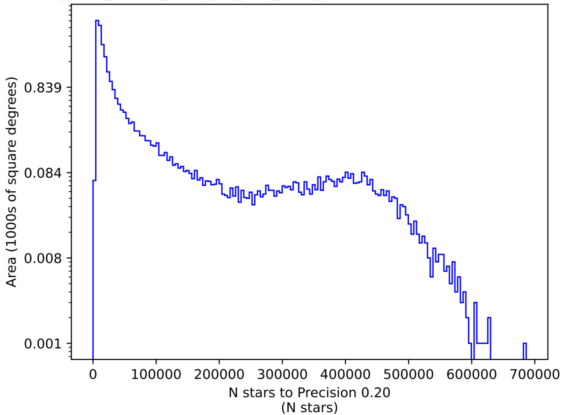
too_elab_heavy_r128_d2_griz_v3.4_10yrs r: N stars to Precision 0.20
