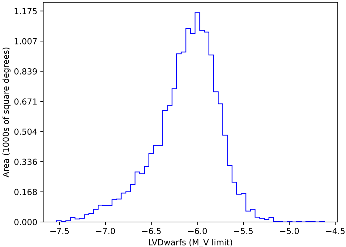
too_elab_heavy_r128_d2_griz_v3.4_10yrs gi: LVDwarfs
