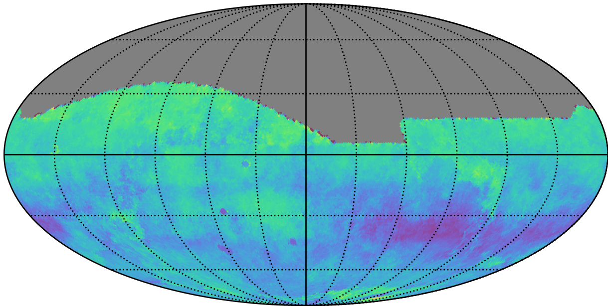
too_elab_heavy_r128_d2_griz_v3.4_10yrs r: Kuiper rotSkyPos
