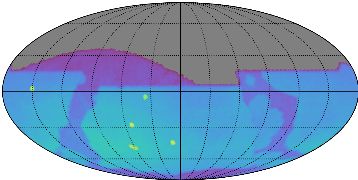
too_elab_heavy_r128_d2_griz_v3.4_10yrs : Brown Dwarf, L4
