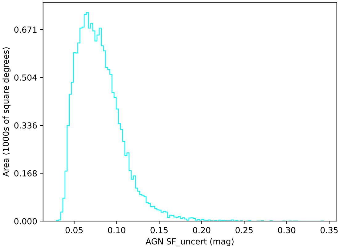
too_elab_heavy_r128_d2_griz_v3.4_10yrs u band: AGN SF_uncert
