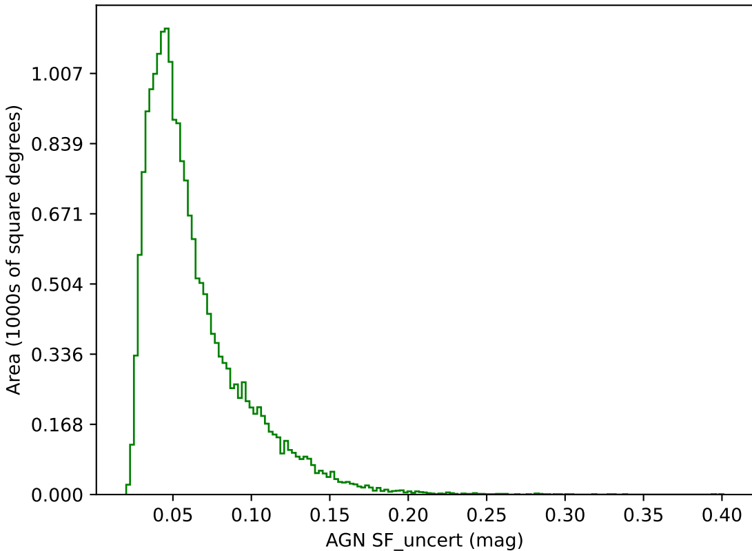
too_elab_heavy_r128_d2_griz_v3.4_10yrs g band: AGN SF_uncert
