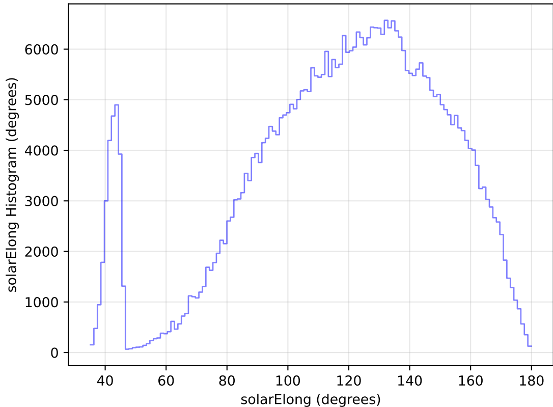
too_elab_heavy_r128_d2_griz_v3.4_10yrs WFD z band: solarElong Histogram
