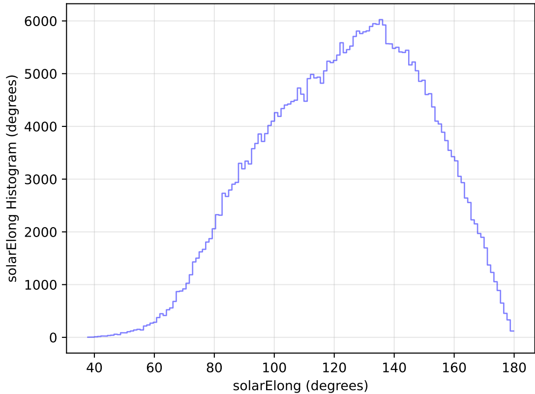
too_elab_heavy_r128_d2_griz_v3.4_10yrs WFD y band: solarElong Histogram
