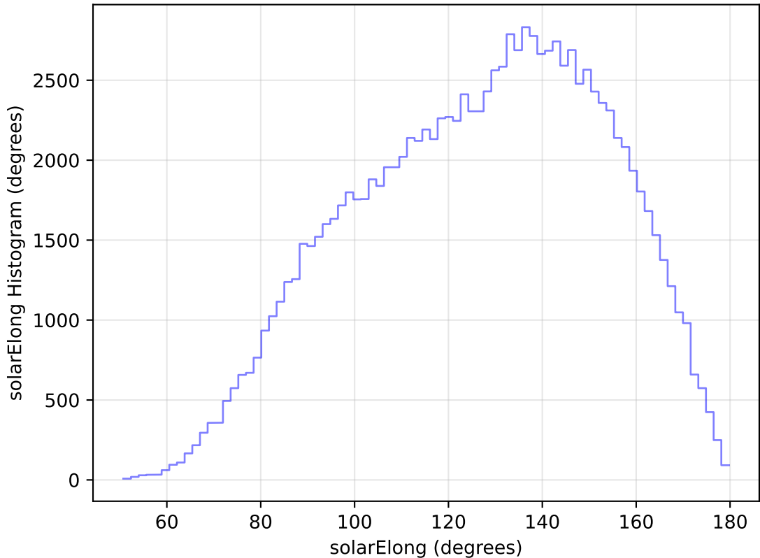
too_elab_heavy_r128_d2_griz_v3.4_10yrs WFD u band: solarElong Histogram
