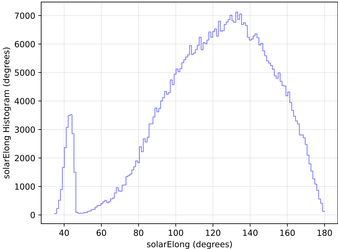
too_elab_heavy_r128_d2_griz_v3.4_10yrs WFD i band: solarElong Histogram
