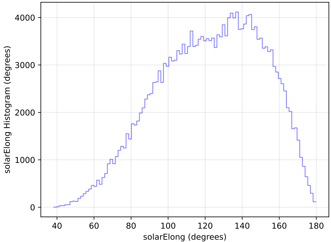
too_elab_heavy_r128_d2_griz_v3.4_10yrs WFD g band: solarElong Histogram
