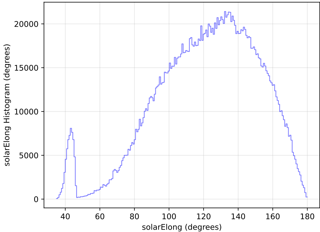
too_elab_heavy_r128_d2_griz_v3.4_10yrs WFD all bands: solarElong Histogram
