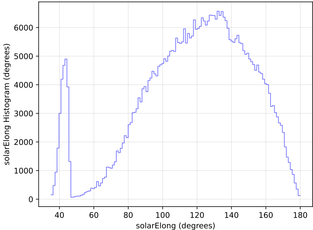
too_elab_heavy_r128_d2_griz_v3.4_10yrs All sky z band: solarElong Histogram
