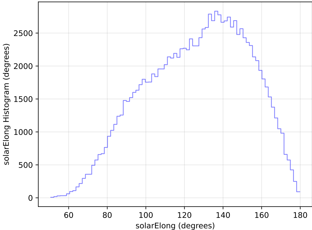
too_elab_heavy_r128_d2_griz_v3.4_10yrs All sky u band: solarElong Histogram
