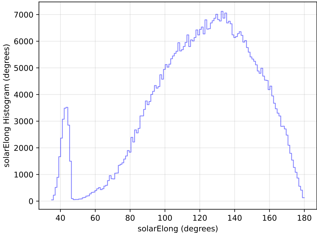
too_elab_heavy_r128_d2_griz_v3.4_10yrs All sky i band: solarElong Histogram
