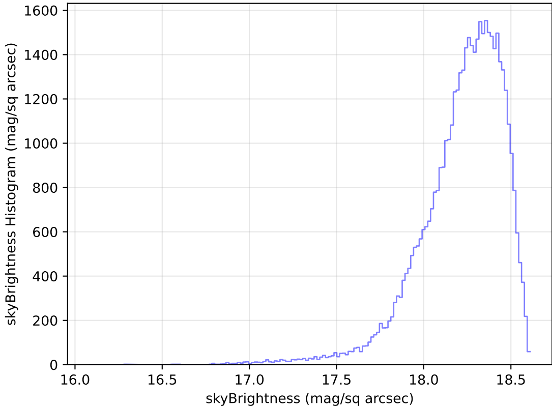
too_elab_heavy_r128_d2_griz_v3.4_10yrs Yr 1 y band: skyBrightness Histogram
