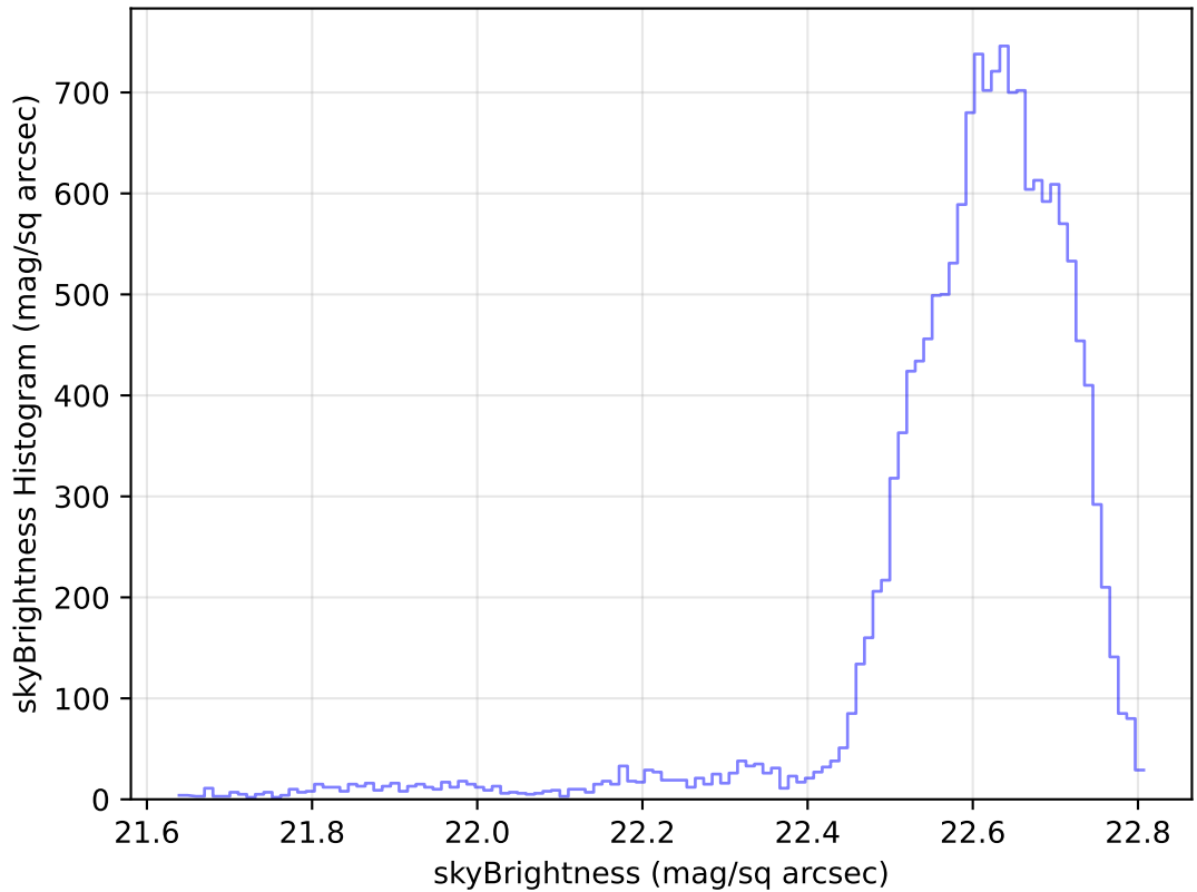
too_elab_heavy_r128_d2_griz_v3.4_10yrs Yr 1 u band: skyBrightness Histogram
