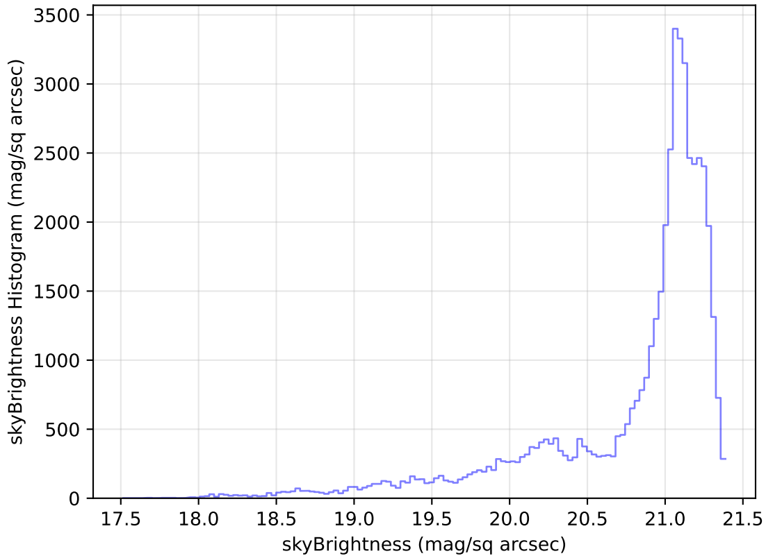
too_elab_heavy_r128_d2_griz_v3.4_10yrs Yr 1 r band: skyBrightness Histogram
