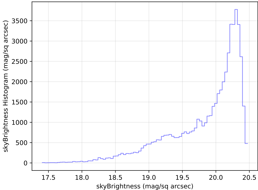
too_elab_heavy_r128_d2_griz_v3.4_10yrs Yr 1 i band: skyBrightness Histogram
