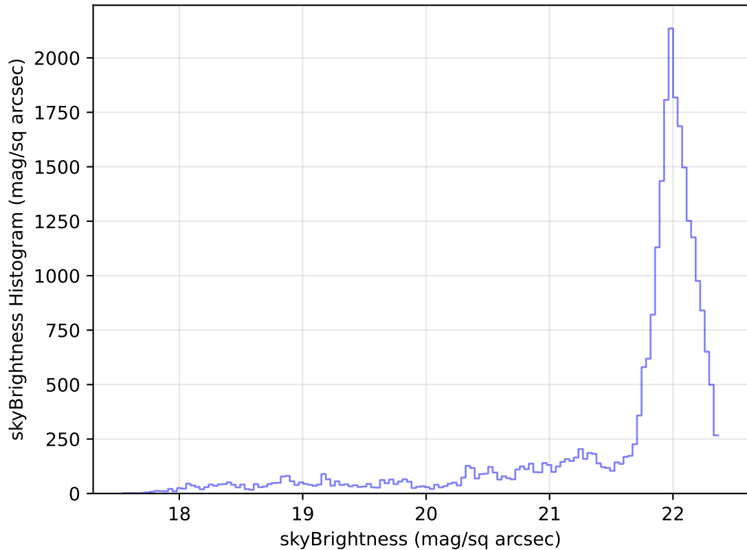
too_elab_heavy_r128_d2_griz_v3.4_10yrs Yr 1 g band: skyBrightness Histogram
