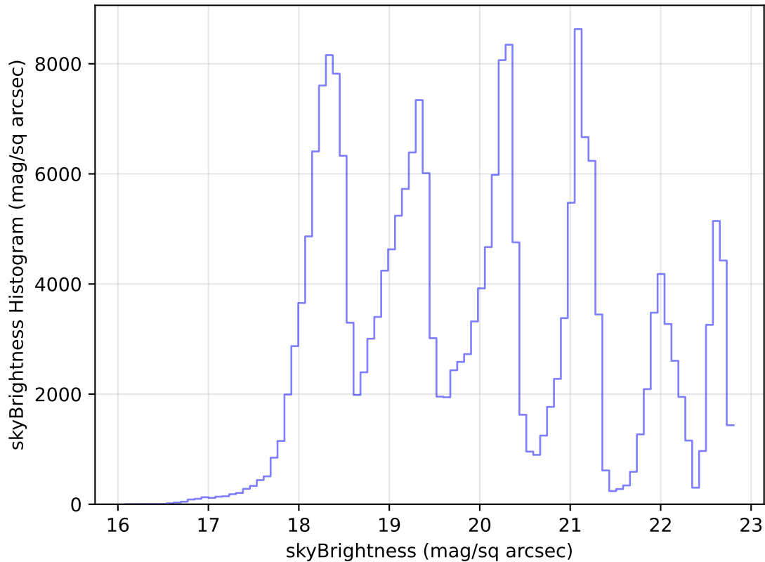
too_elab_heavy_r128_d2_griz_v3.4_10yrs Yr 1 all bands: skyBrightness Histogram
