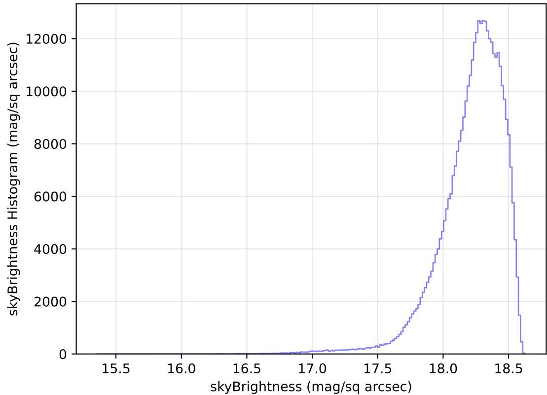
too_elab_heavy_r128_d2_griz_v3.4_10yrs WFD y band: skyBrightness Histogram
