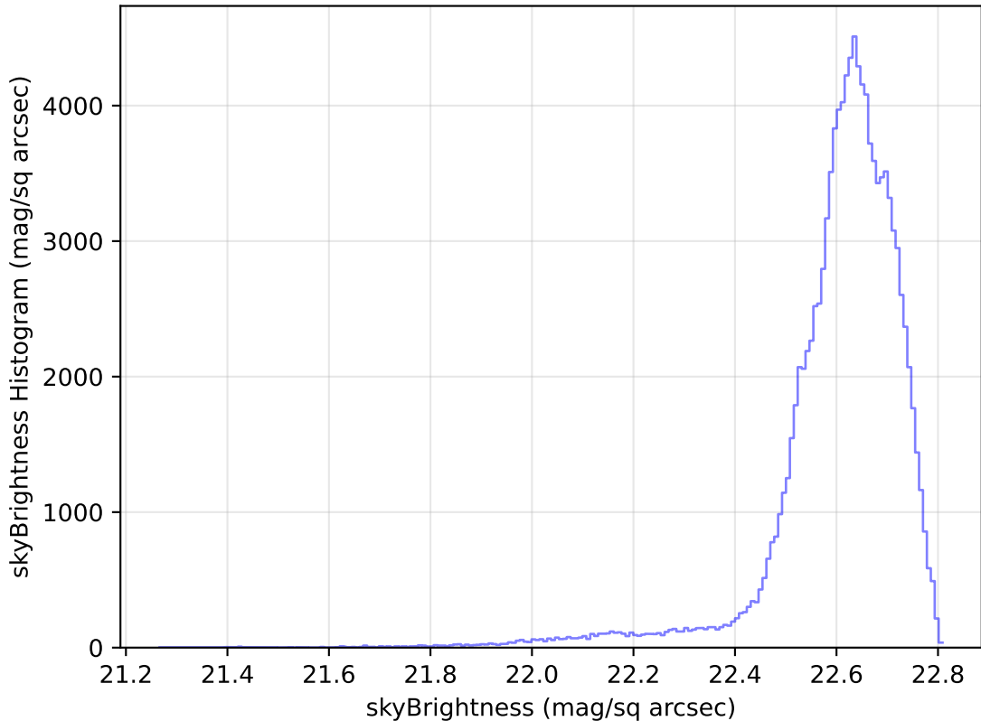
too_elab_heavy_r128_d2_griz_v3.4_10yrs WFD u band: skyBrightness Histogram
