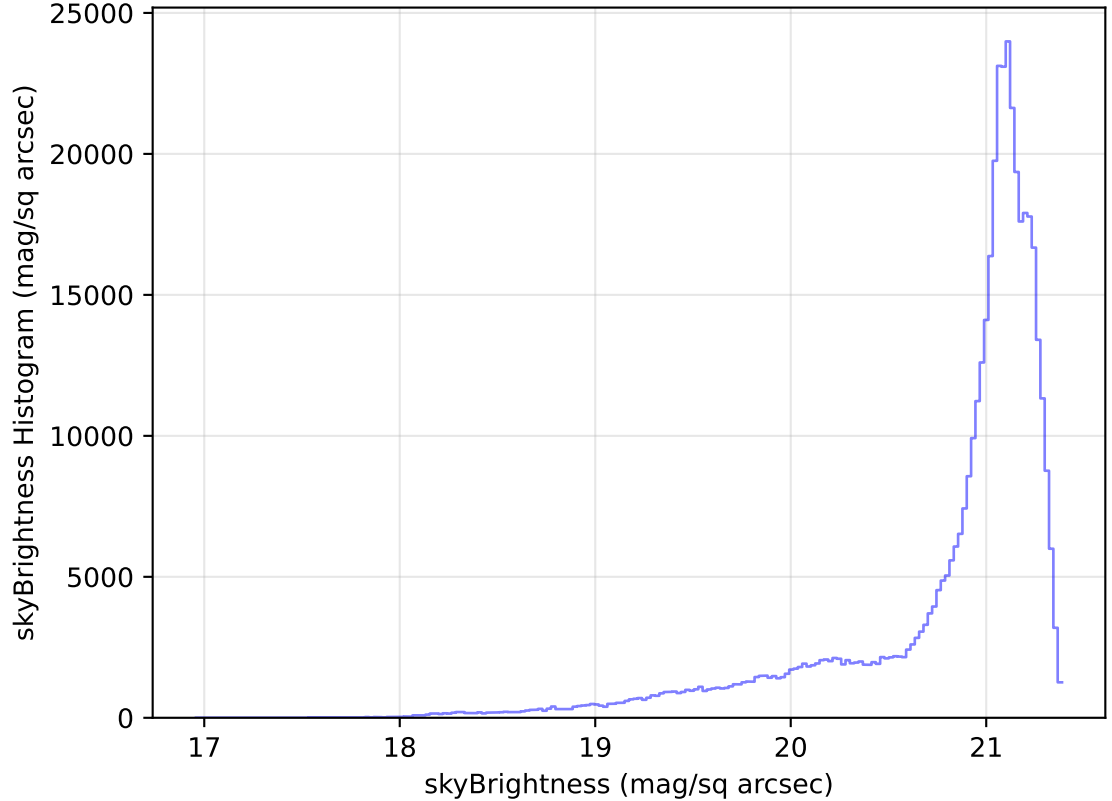
too_elab_heavy_r128_d2_griz_v3.4_10yrs WFD r band: skyBrightness Histogram
