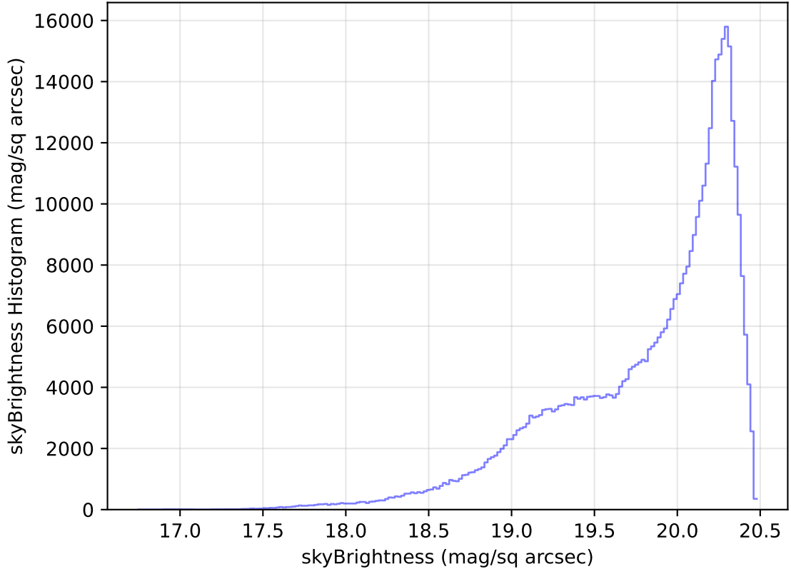
too_elab_heavy_r128_d2_griz_v3.4_10yrs WFD i band: skyBrightness Histogram
