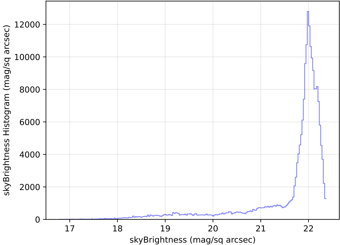
too_elab_heavy_r128_d2_griz_v3.4_10yrs WFD g band: skyBrightness Histogram
